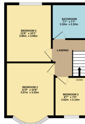
1ST FLOOR 439 sq. ft. (40.8 sq.m.) approx.
