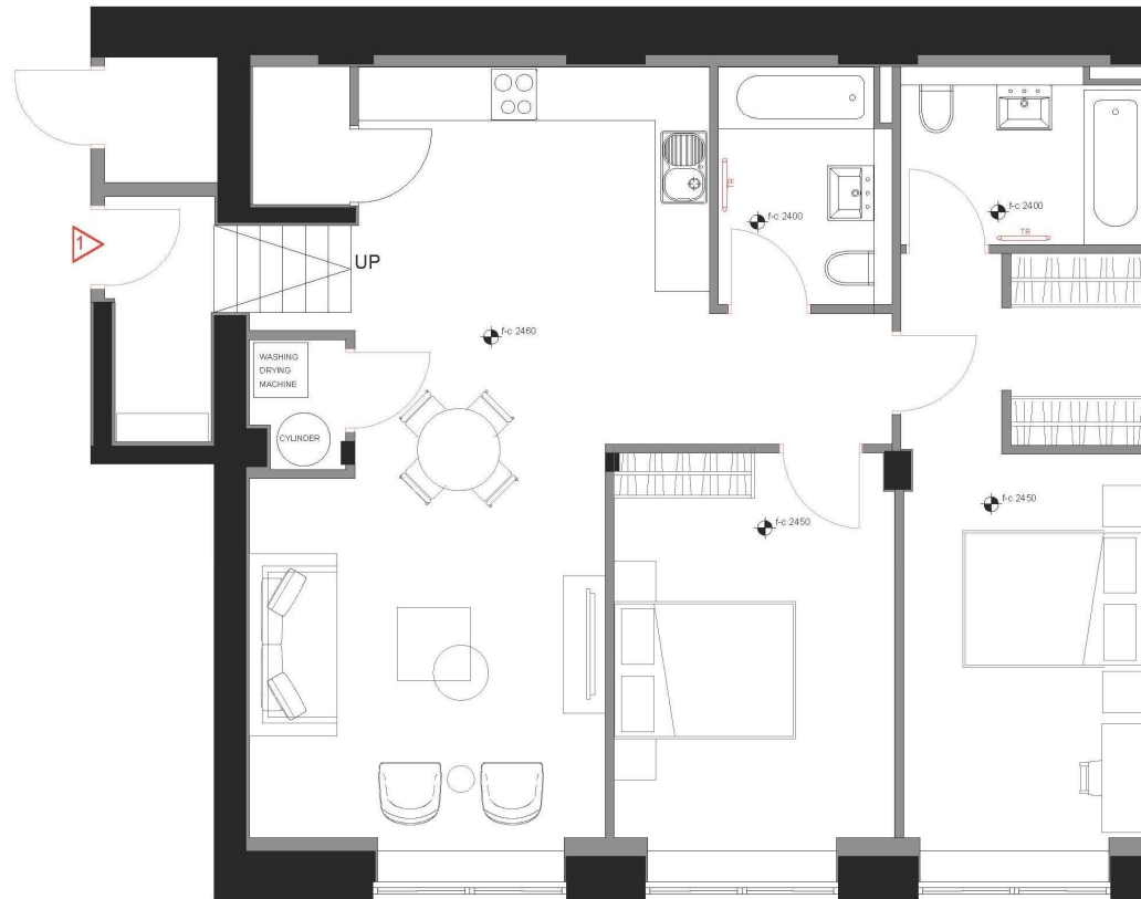
GA Plan - Proposed Apartment 1 1 : 50
