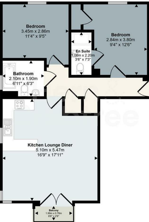
Floorplan
