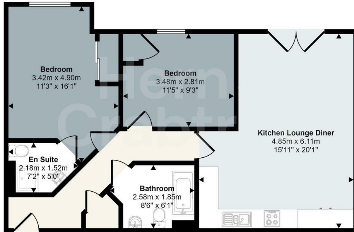
Floorplan
