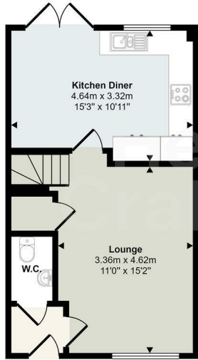
Ground Floor Approx 37 sq m / 397 sq ft
