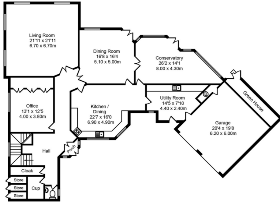
Main Ground Floor Approx. Floor Area 2665 Sq.Ft (247.6 Sq.M.)
