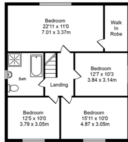
First Floor Approx. Floor Area 924 Sq.Ft (85.8 Sq.M.)
