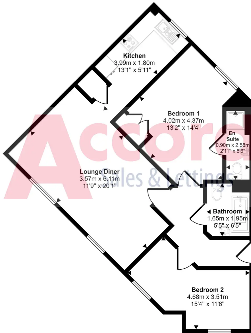
Floorplan
