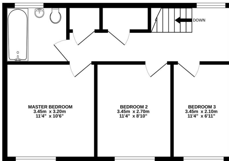
1ST FLOOR
