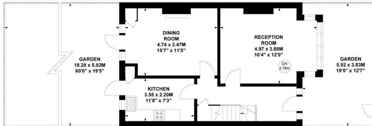
Ground Floor
