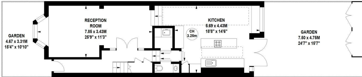
Ground Floor
