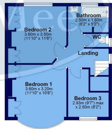
First Floor Approx. 42.6 sq. metres (458.3 sq. feet)
