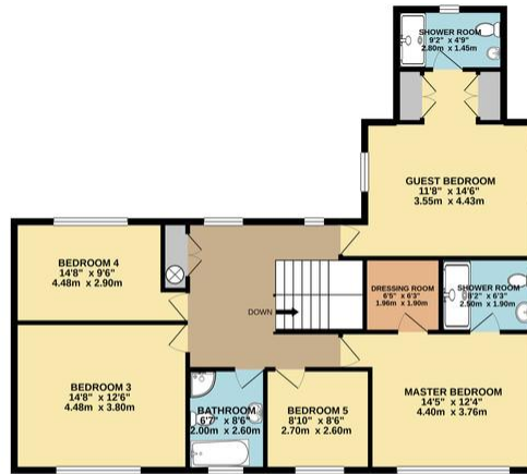
1ST FLOOR 1135 sq.ft. (105.4 sq.m.) approx.
