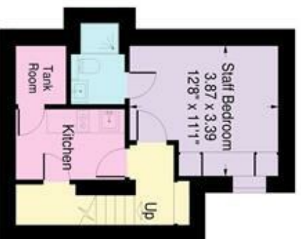
Basement
