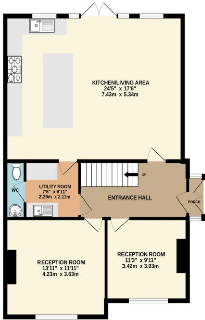
GROUND FLOOR 879 sq.ft. (81.6 sq.m.) approx.
