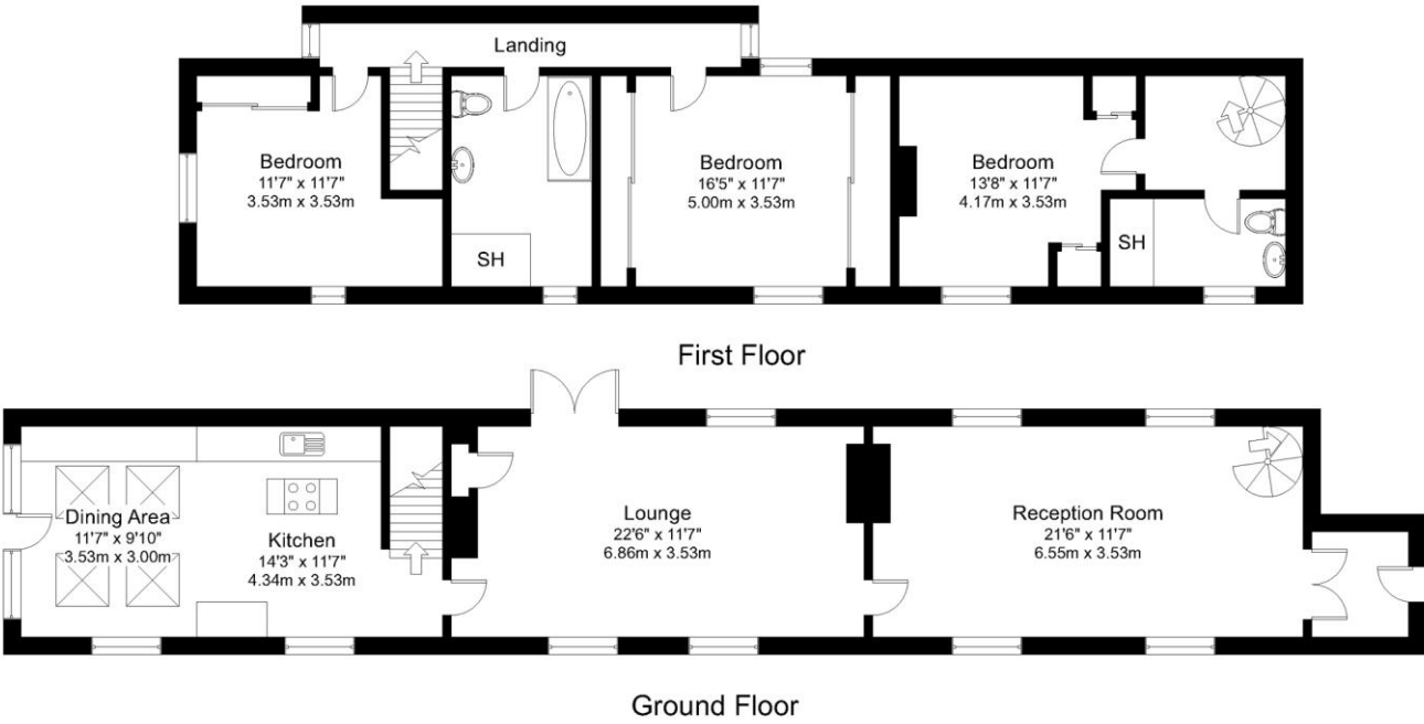
Gross internal floor area (approx.): 151.4 sq m (1,630 sq ft) Not to Scale. Copyright © Apex Plans. For illustrative purposes only.
