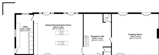
Ground Floor Floor area 141.1 sq.m. (1,519 sq.ft.)
