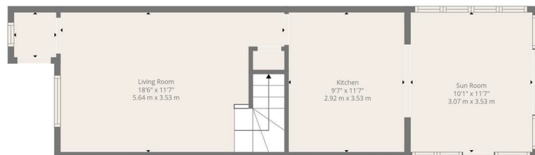
Floor 1
