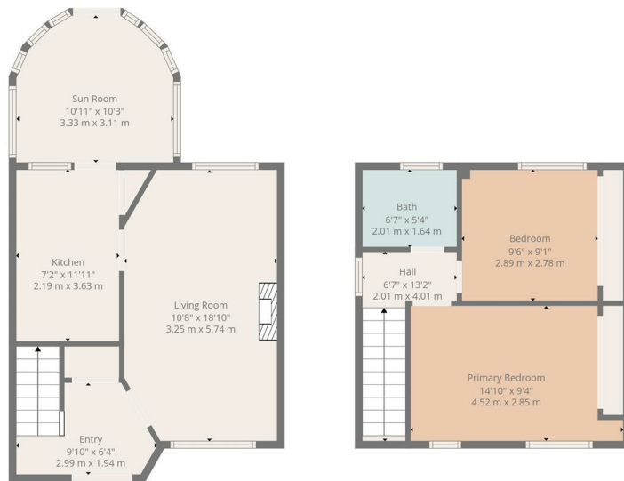
Floor 2
