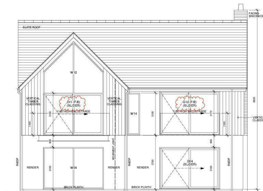
PROPOSED NORTH WEST ELEVATION
