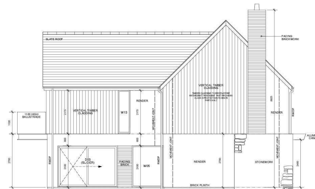
PROPOSED SOUTH-WEST ELEVATION
