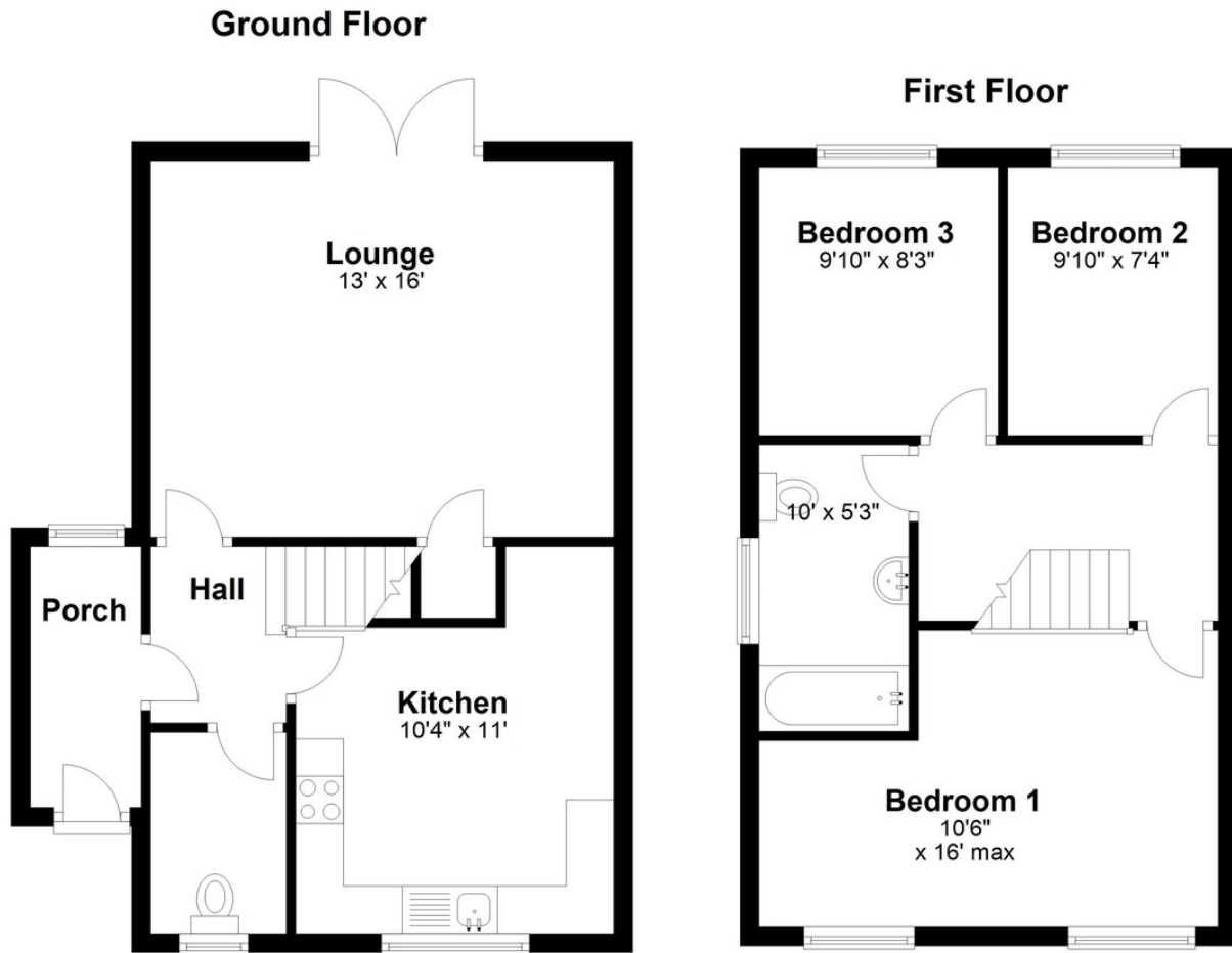
Floor plan mirror image of No 27.
