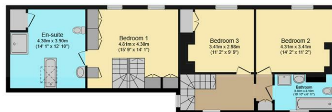
First Floor Floor area 85.7 sq.m. (923 sq.ft.)
