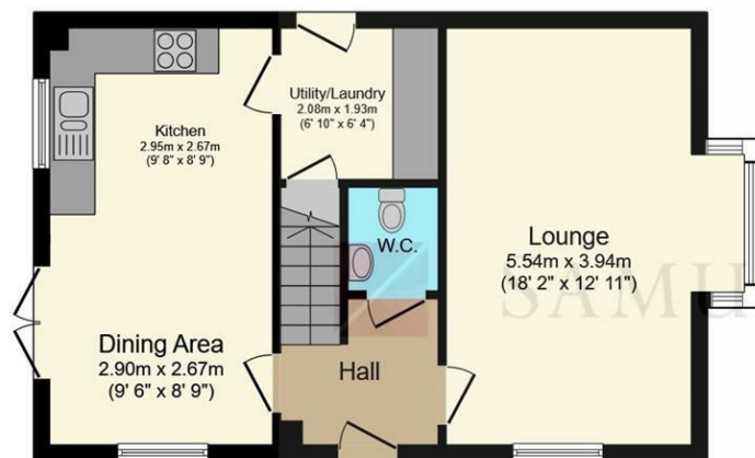
Ground Floor Floor area 47.9 m 2 (515 sq.ft.)
