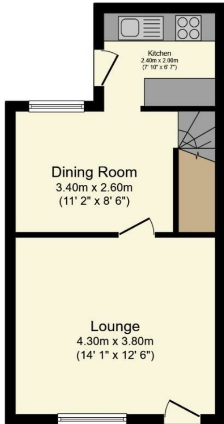
Ground Floor Floor area 33.0 sq.m. (355 sq.ft.)
