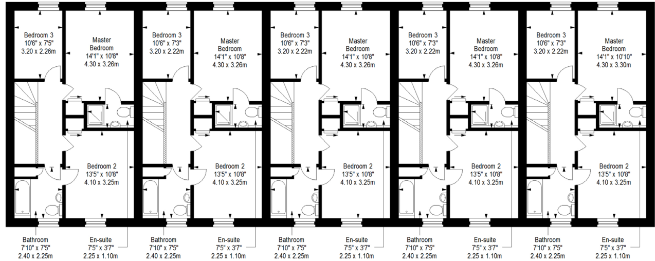
Ground Floor Approx. 264.8 sq. metres (2850.4 sq. feet)
