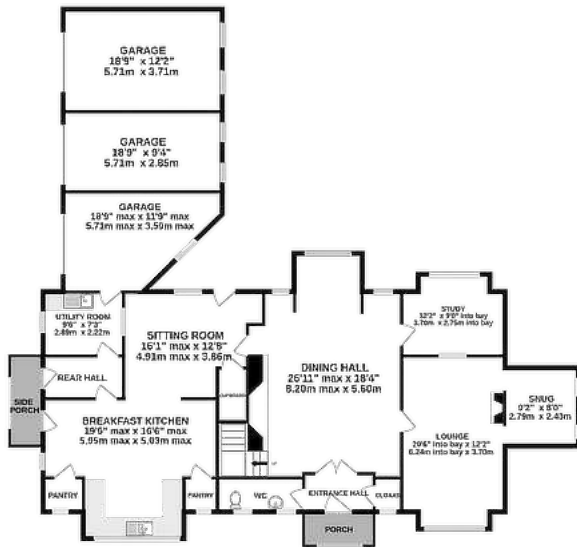
GROUND FLOOR 2136 sq.ft. (198.5 sq.m.) approx.
