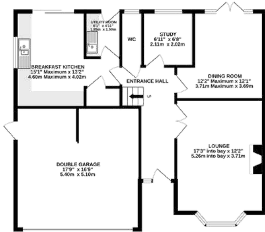
GROUND FLOOR 968 sq.ft. (89.9 sq.m.) approx.
