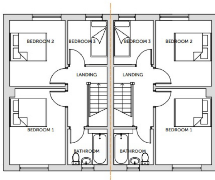
Proposed First Floor Plan 1:50
