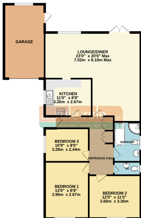
GROUND FLOOR 1189 sq.ft. (110.4 sq.m.) approx.
