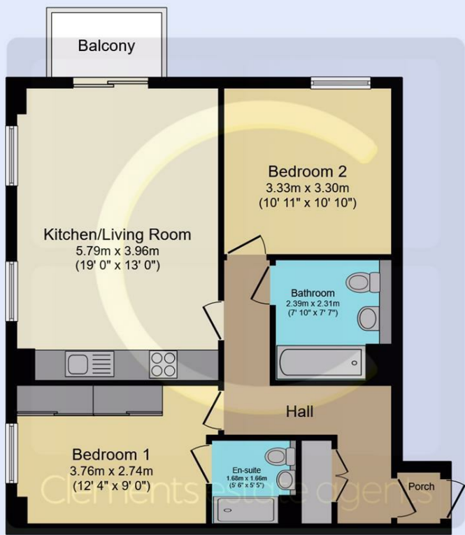
Floor Plan
