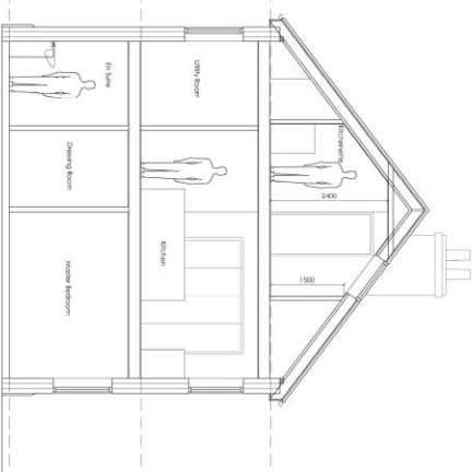
Typical Section 1:50
