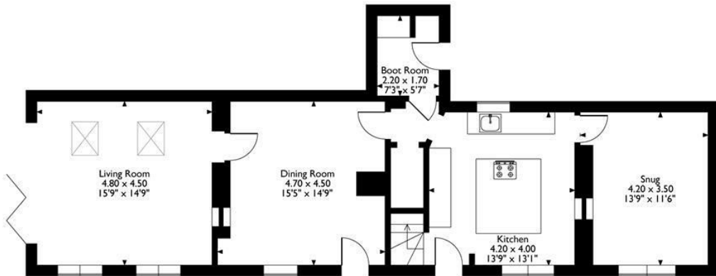
Ground Floor
