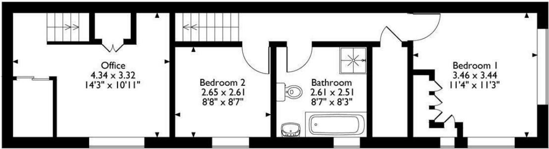
First Floor
