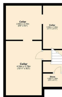
Lower Ground Floor Approx. 29.7 sq. metres (319.5 sq. feet)
