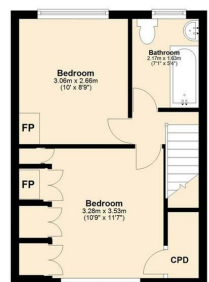
First Floor Approx. 28.2 sq. metres (303.6 sq. feet)
