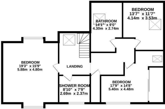
1ST FLOOR
