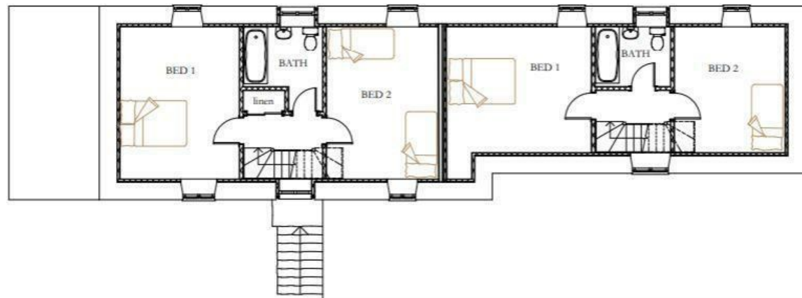
BARN F FLOOR - PROPOSED 1:100
