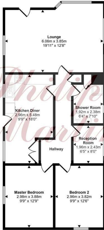
Floorplan
