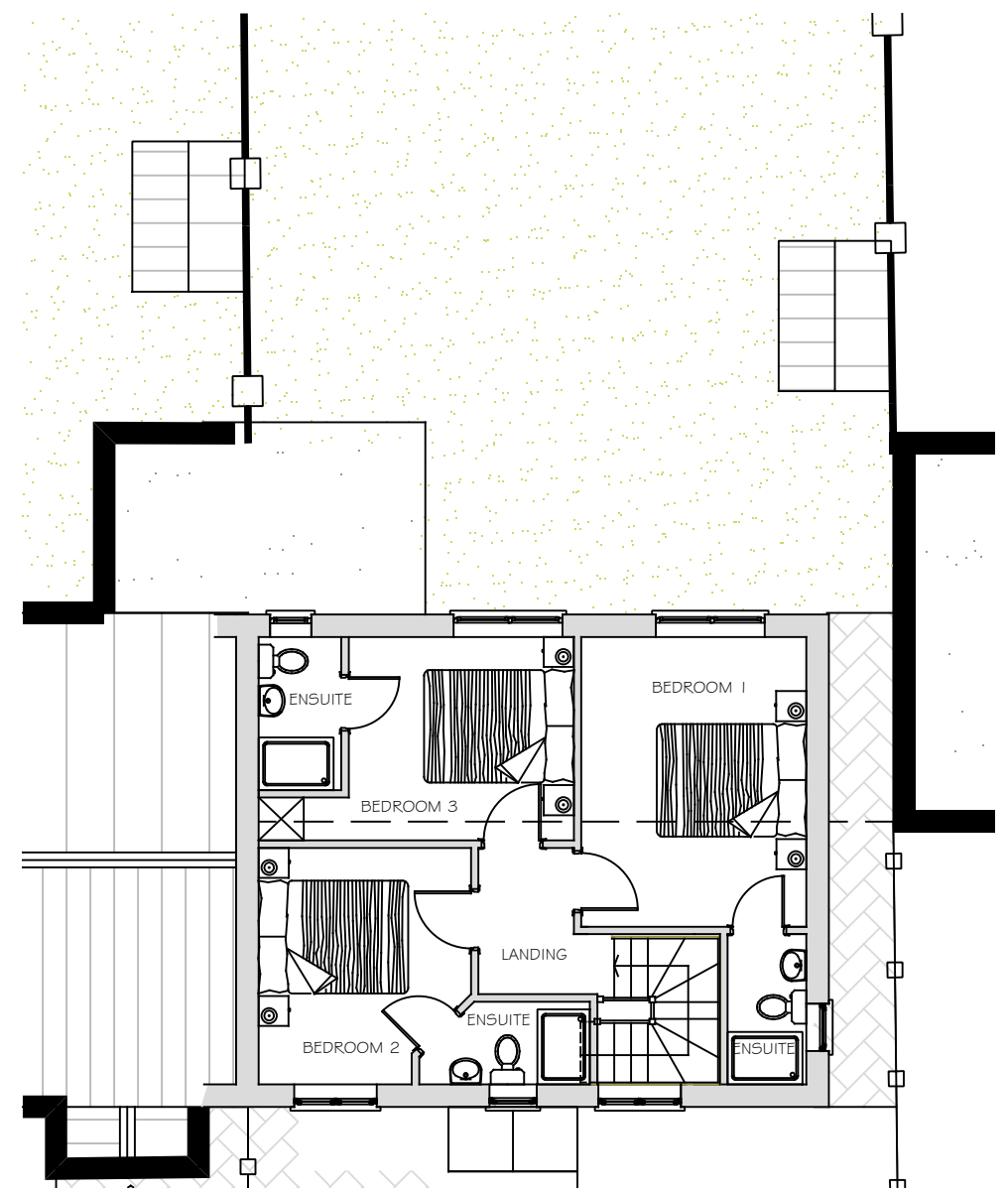
FIRST FLOOR PLAN Scale 1/100 @ A3 As Proposed
