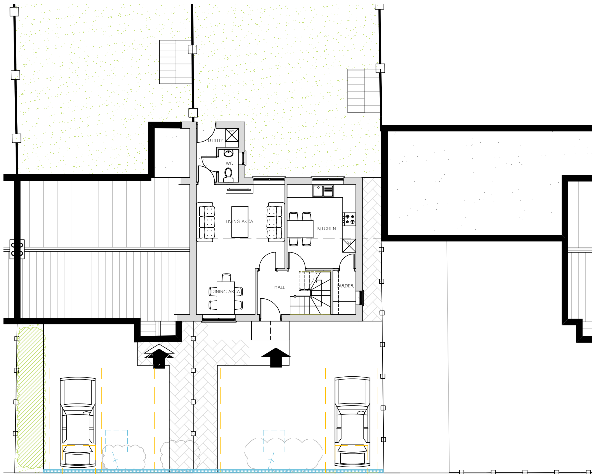
GROUND FLOOR PLAN Scale 1/100 @ A3 As Proposed
