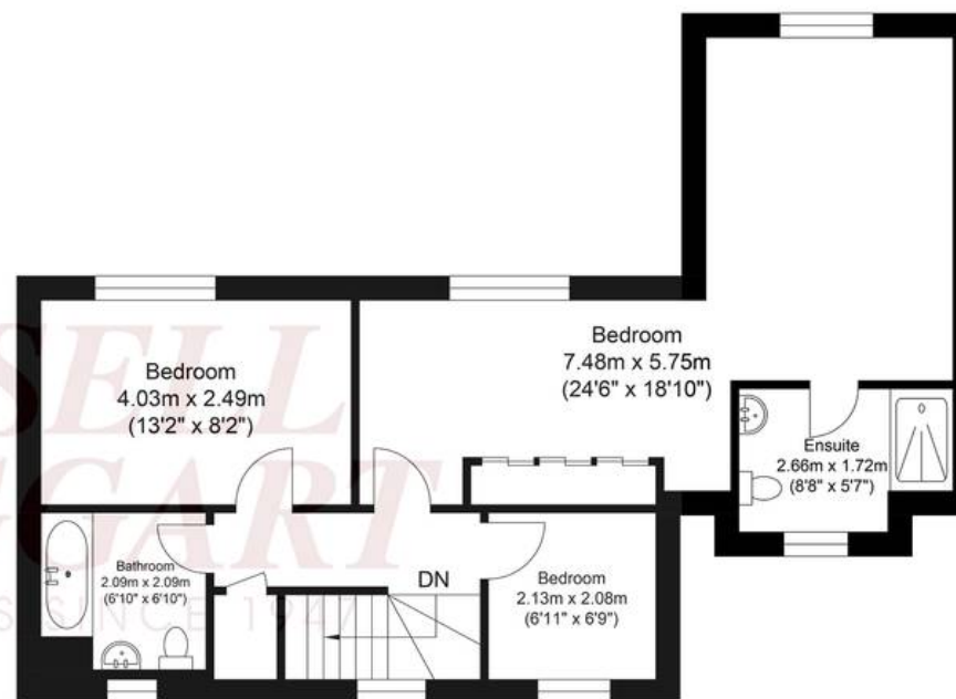
First Floor Approximate Floor Area 626.89 sq ft (58.24 sq m)
