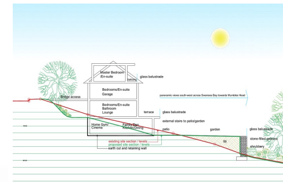
BUILDING PLOT 3 CONCEPTUAL SKETCH SCHEME and SITE SECTION PEARSON WAY, GARTHOR, NEATH Scale 1:100 compton group
