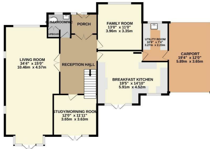
GROUND FLOOR 1539 sq.ft. (143.0 sq.m.) approx.
