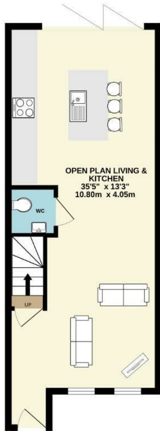
GROUND FLOOR 439 sq.ft. (40.8 sq.m.) approx.
