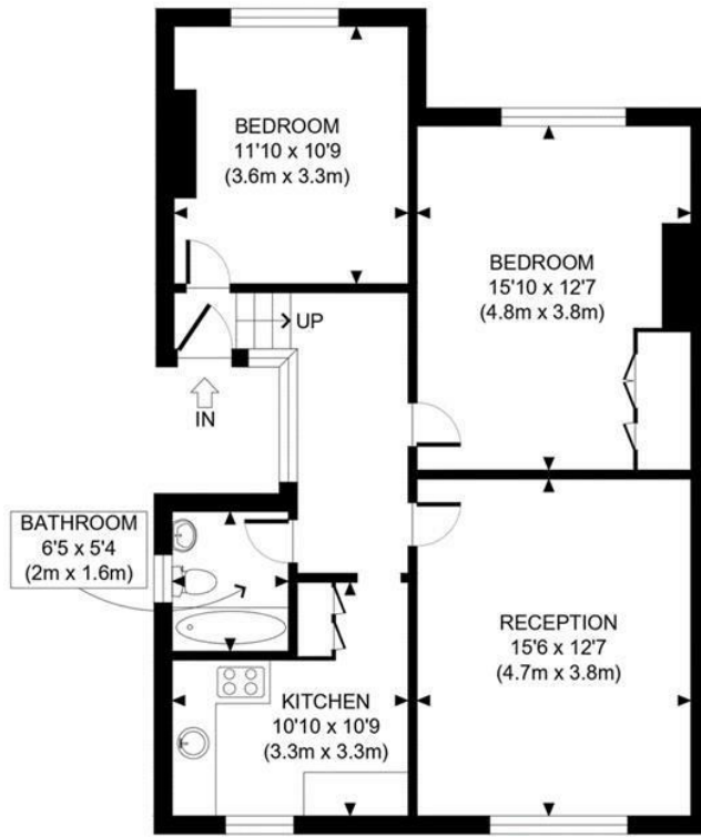
SECOND FLOOR GROSS INTERNAL FLOOR AREA 762 SQ FT
