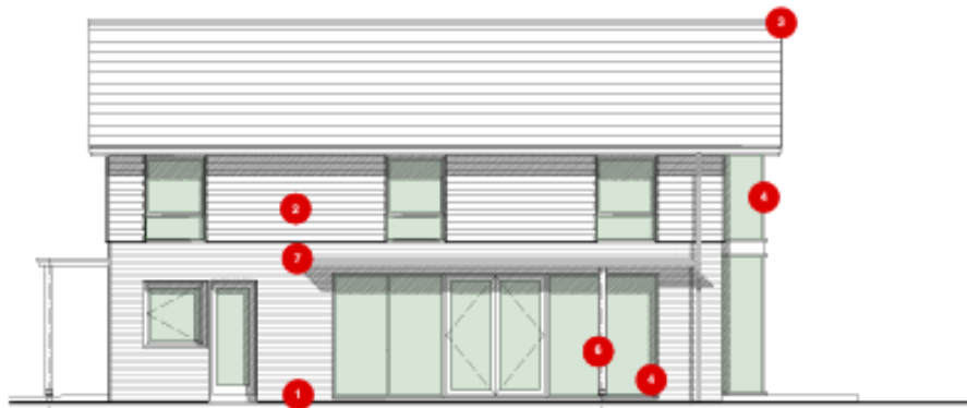
1 NORTH ELEVATION SCALE - 1:100
