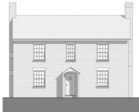
Plot 1 - Front Elevation 1 : 100
