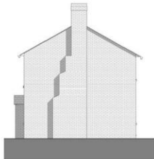
Plot 1 - Side Elevation B 1 : 100
