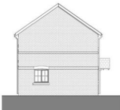
Plot 3 - Side Elevation B 1 : 100
