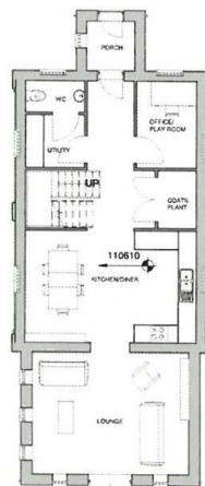
Ground floor- Proposed conversion 1 : 100
