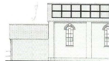
SE elevation- Proposed conversion 1 : 100
