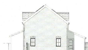
South east elevation- New build 1 : 100
