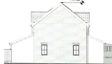
North west elevation- New build 1 : 100
