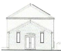
SW elevation- Proposed conversion 1 : 100
