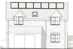
South west elevation- New build 1 : 100
