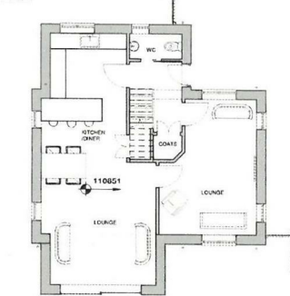
Ground floor- new dwelling 1 : 100
