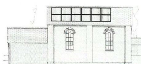
SE elevation- Proposed conversion 1 : 100
