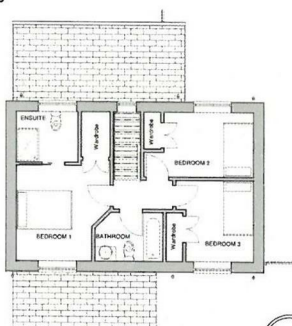
First floor- New dwelling 1 : 100
