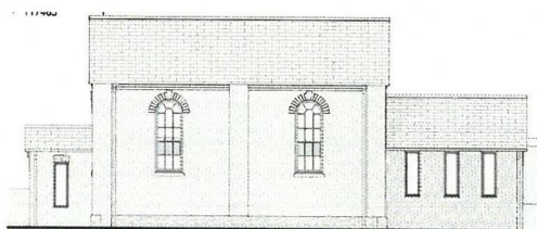
SW elevation- Proposed conversion 1 : 100
