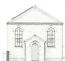
NE elevation- Proposed conversion 1 : 100
