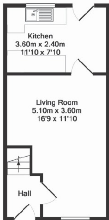
Ground Floor Approx. Floor Area 27.0 Sq.M. (291 Sq.Ft.)
