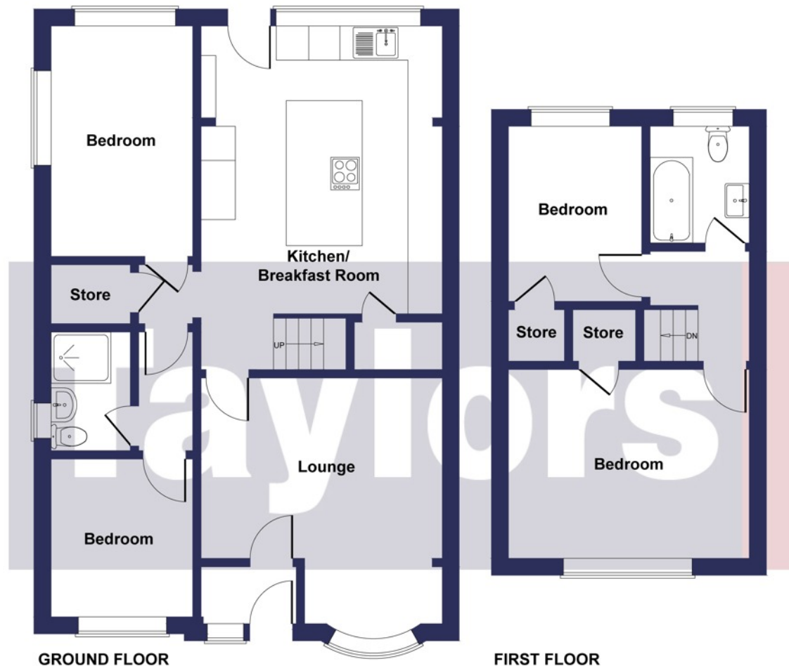
GROUND FLOOR
