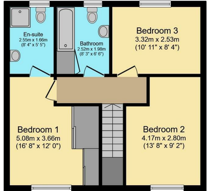
First Floor Floor area 48.0 m 2 (517 sq.ft.)
